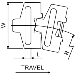
HS-880-EL BO (Side Flexing Plastic Chain)
